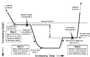
FIG. 1 Rockwell Hardness Test Method (Schematic Diagram)
