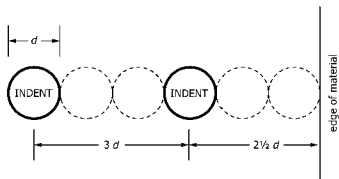
FIG. 3 Schematic of Minimum Indentation Spacing
