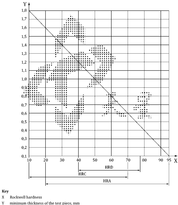
Figure B.1 — Test with diamond cone indenter (scales A, C, and D)
